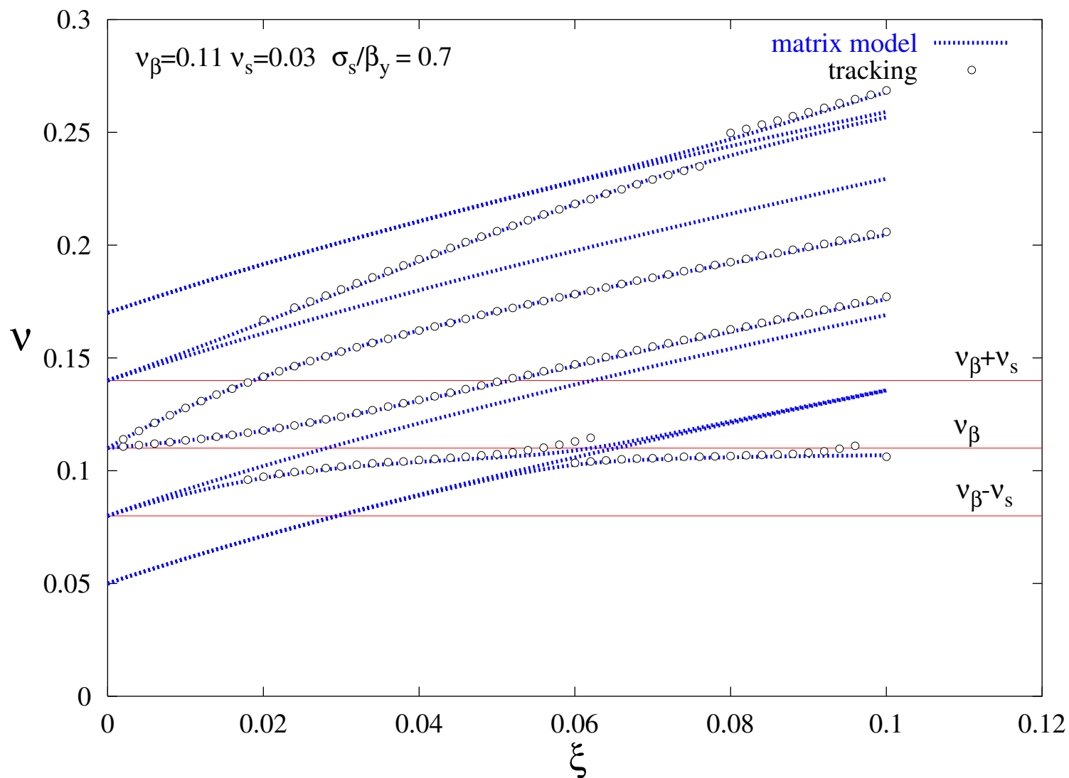
Coherent synchro-betatron mode tunes vs. the beam-beam parameter \xi . Comparison of matrix calculation and tracking with Gaussian distribution in the synchrotron phase space.
