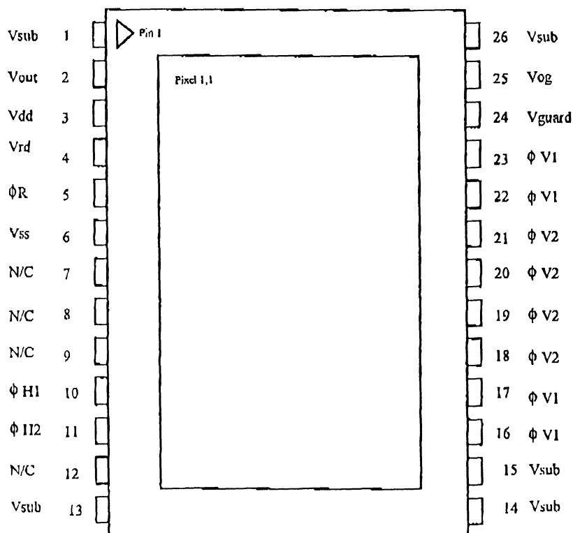
Figure 3 - Package Pin Designations
