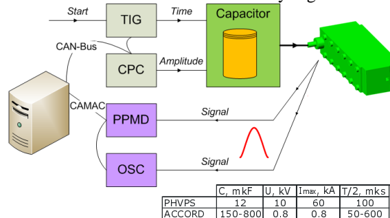
Figure 2. Schematic and main parameters of pulsed power sources. PPMD - pulsed parameters measuring device - integrating ADC.
